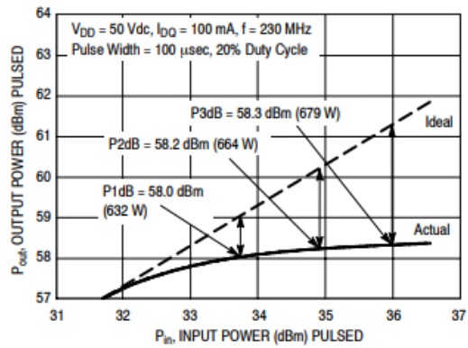
Figure 4. Pulsed Output Power versus Input Power
