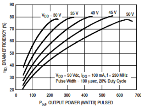
Figure 7. Pulsed Drain Efficiency versus Output Power
